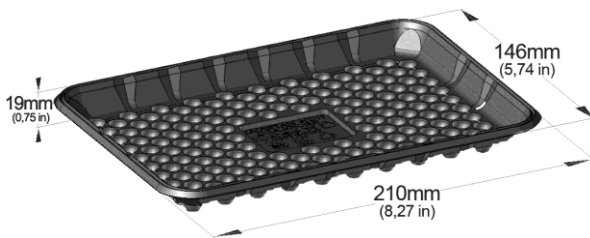
Vista Isométrica / Isometric view
